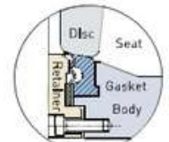
HF-TF Teflon / St. steel 316 Fire Safe-Teflon + Metal
