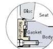
HF-FM INCONEL 625 / St. steel 316 Flat Metal Seat
