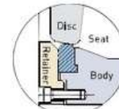
HF-R EPDM / NBR / VITON Rubber Seat
