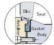
HF-SM SF, St. steel 316 / MONEL Solid Metal Seat
