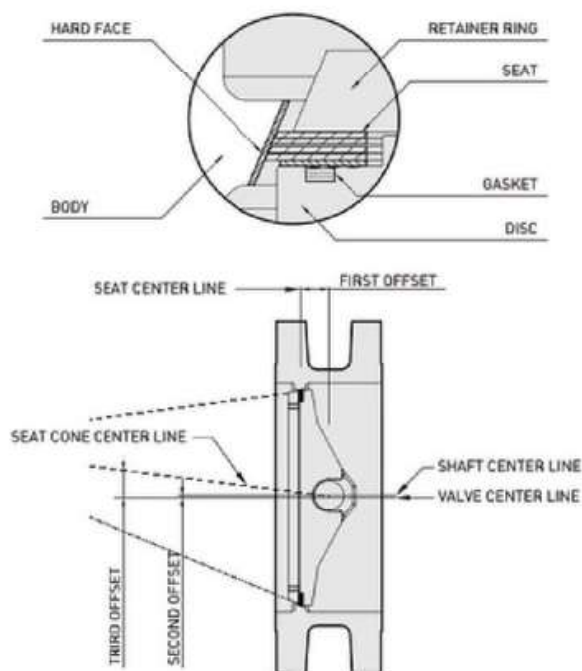
TRIPLE-OFFSET GEOMETRY
